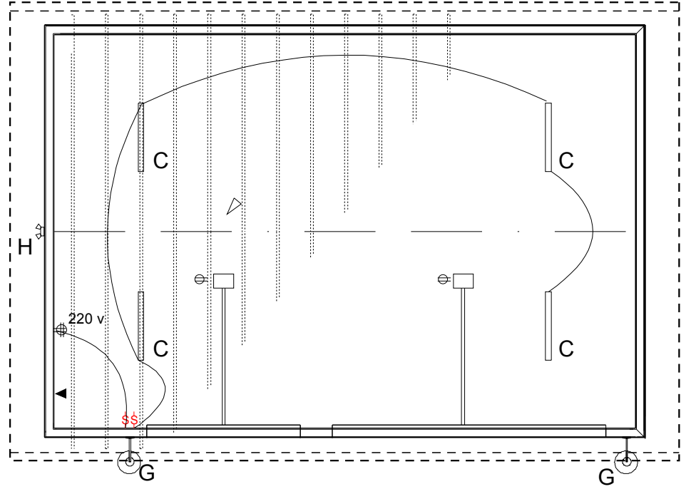
3 GARAGE-POWER-LIGHT A-16 Scale 1/8"=1'-0" 34FT-GAR_POWER-LIGHT
