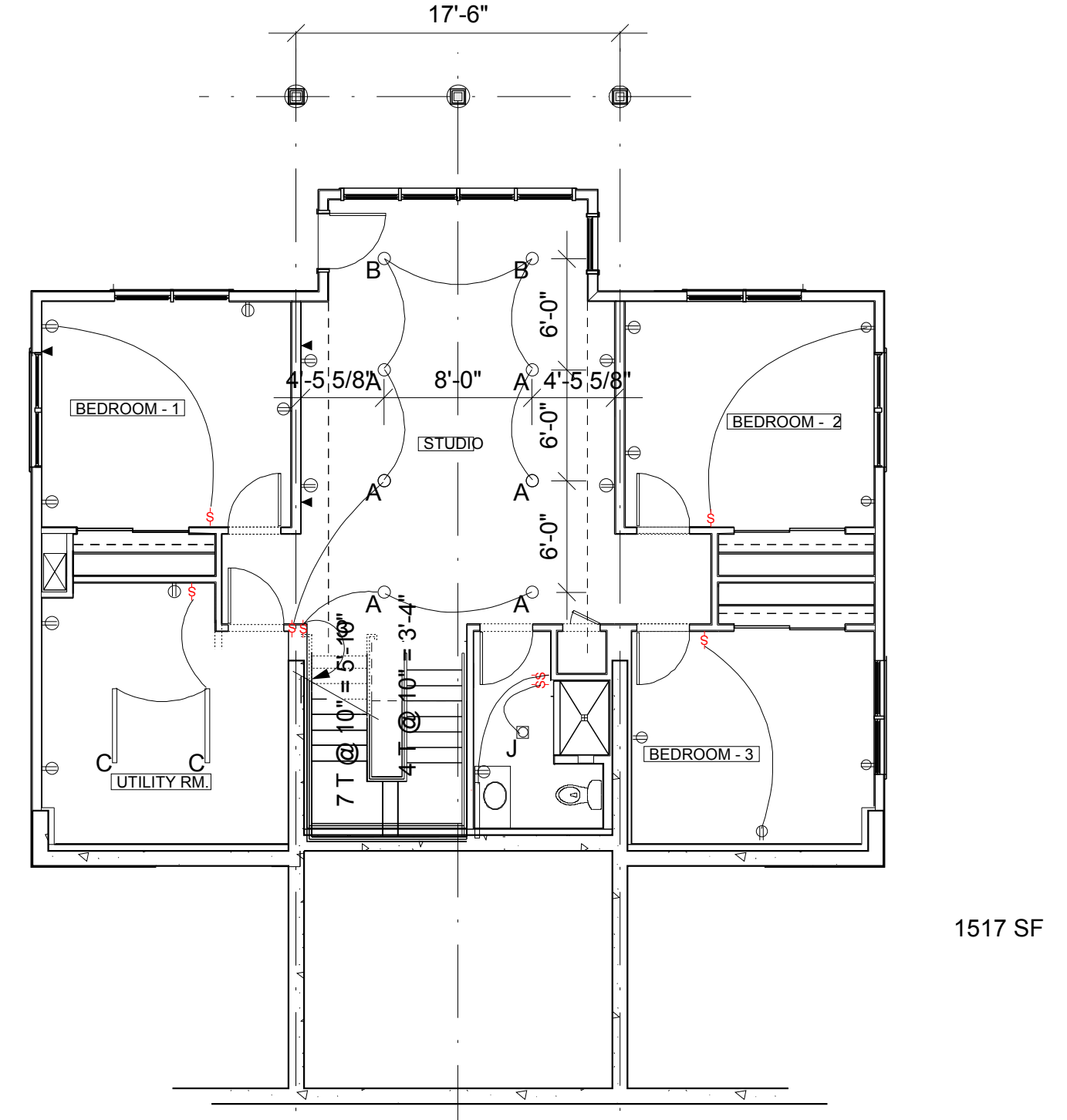
2 GROUND FLOOR POWER -LIGHTING A-16 Scale 1/8"=1'-0" LEV-LOWER-PLN_POWER-LIGHT
