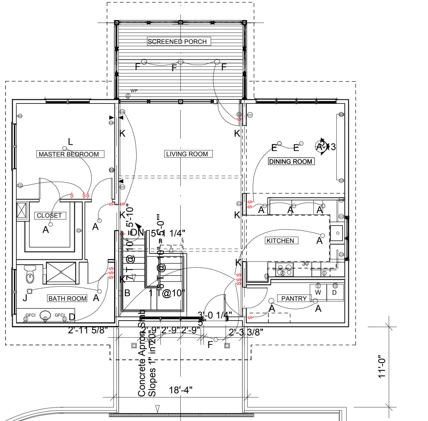
1 FIRST FLOOR POWER -LIGHTING A-16 Scale 1/8"=1'-0" LEV-1-FL_POWER-LIGHT
