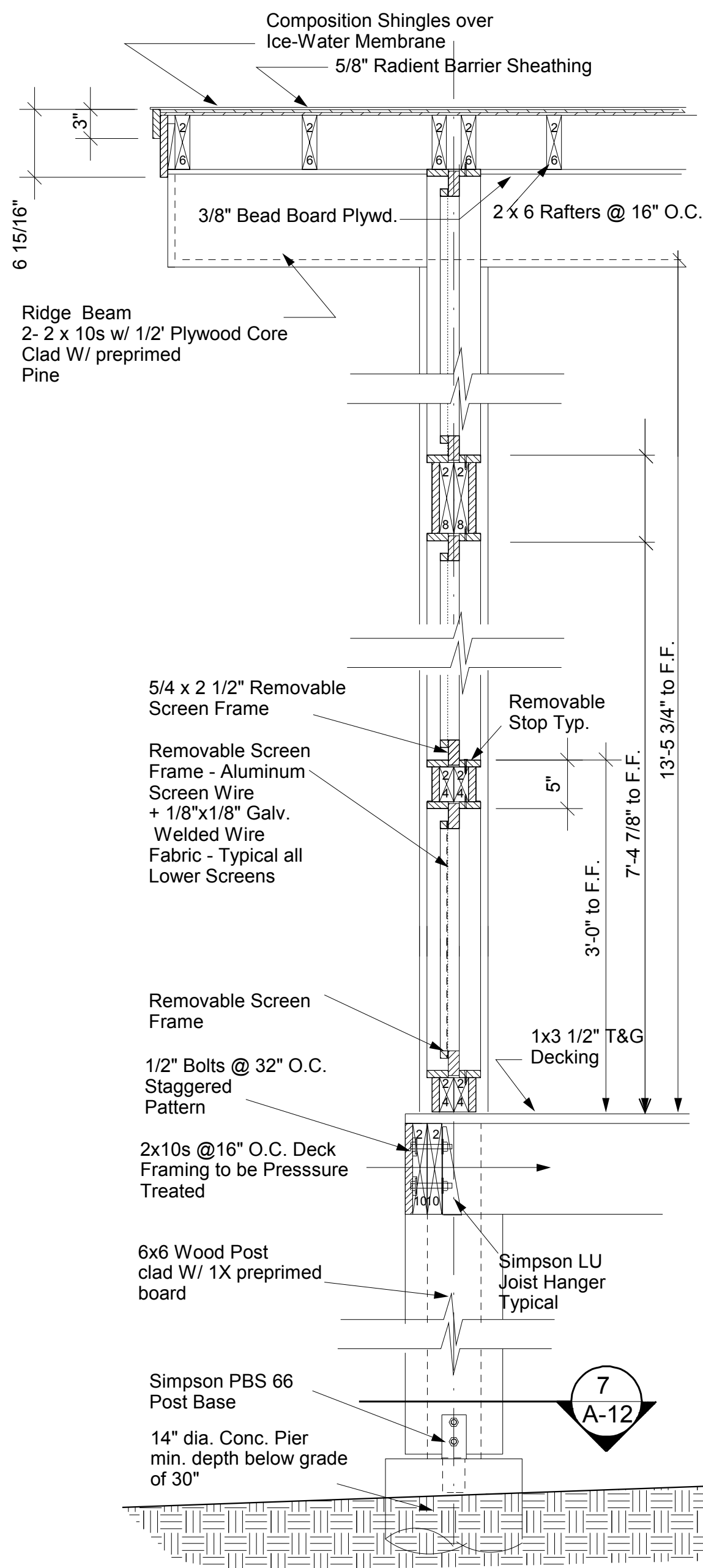
3 SECT. WEST SCREEN WALL A-12 Scale 1"=1'-0" SCREEN-WEST-SECT-12
