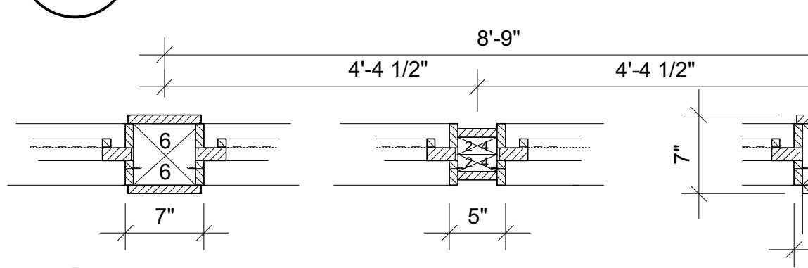
5 SCREEN POST DETAIL A-12 Scale 1"=1'-0" POST-DETS
