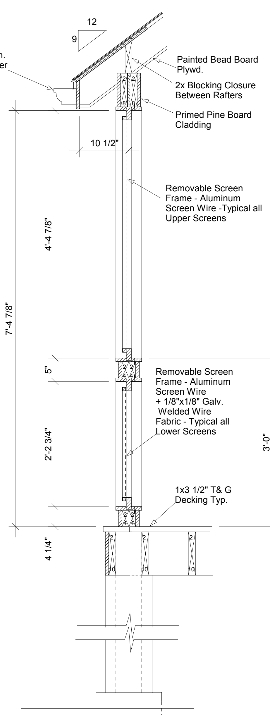
4 SECT. NORTH & SOUTH SCREEN WALL A-12 Scale 1"=1'-0" SCREEN-N-S-SECT-12
