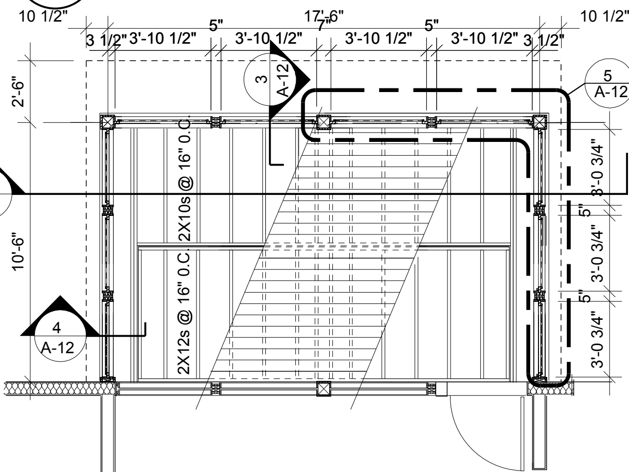
2 SCREENED PORCH - PLAN A-12 Scale 1/4"=1'-0" SCREEN-PORCH-PLN
