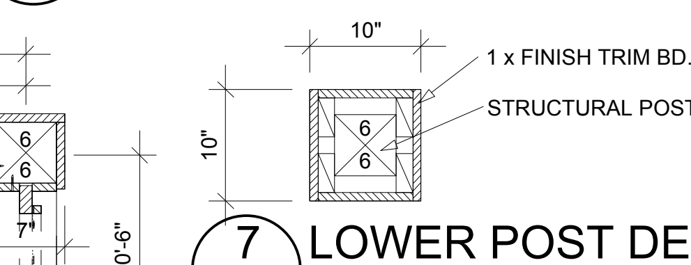
7 LOWER POST DET. A-12 Scale 1"=1'-0"
