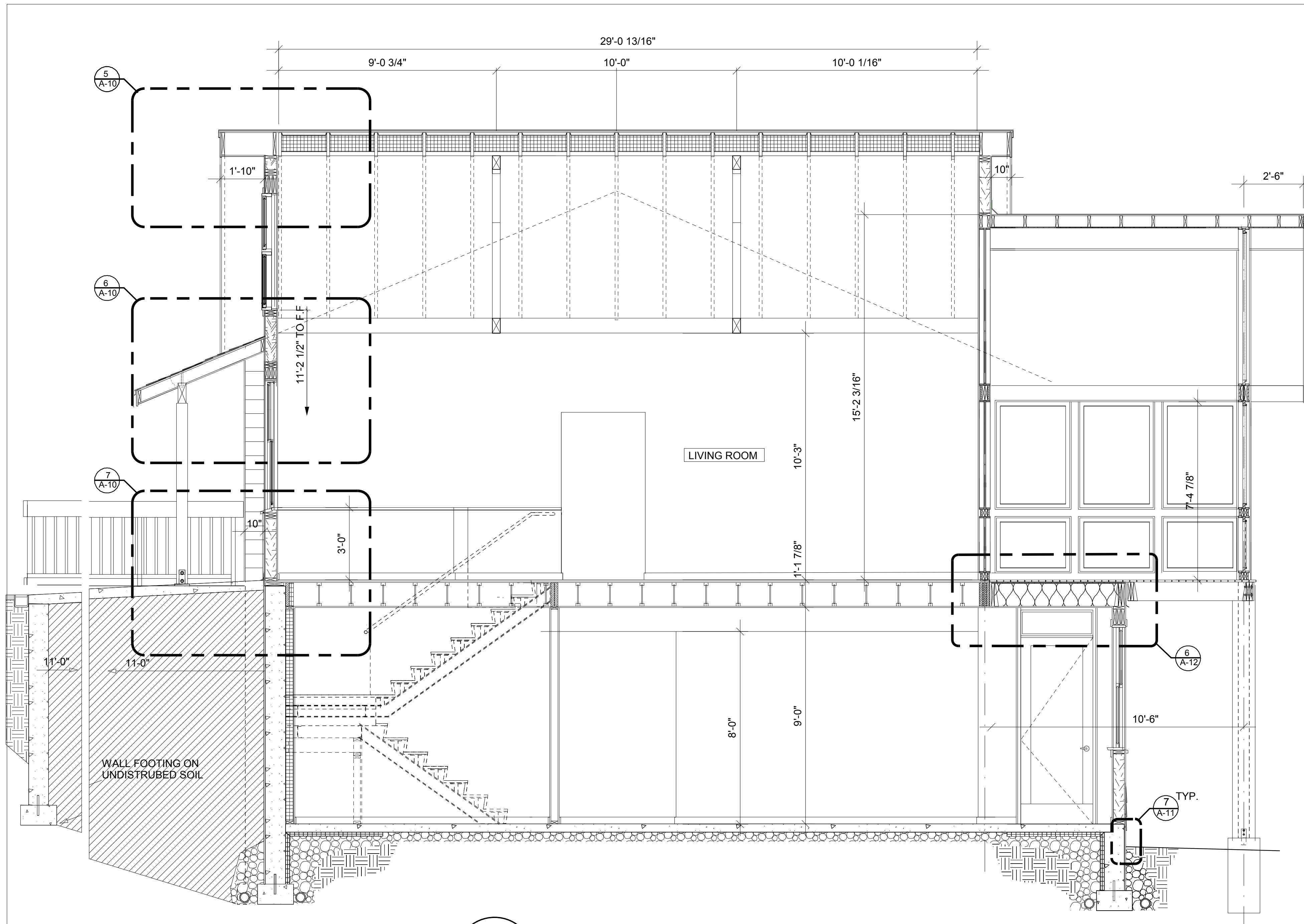
1 EAST to WEST -SECTION # 2 A-9 Scale 3/8"=1'-0" E-W-SECT-2
