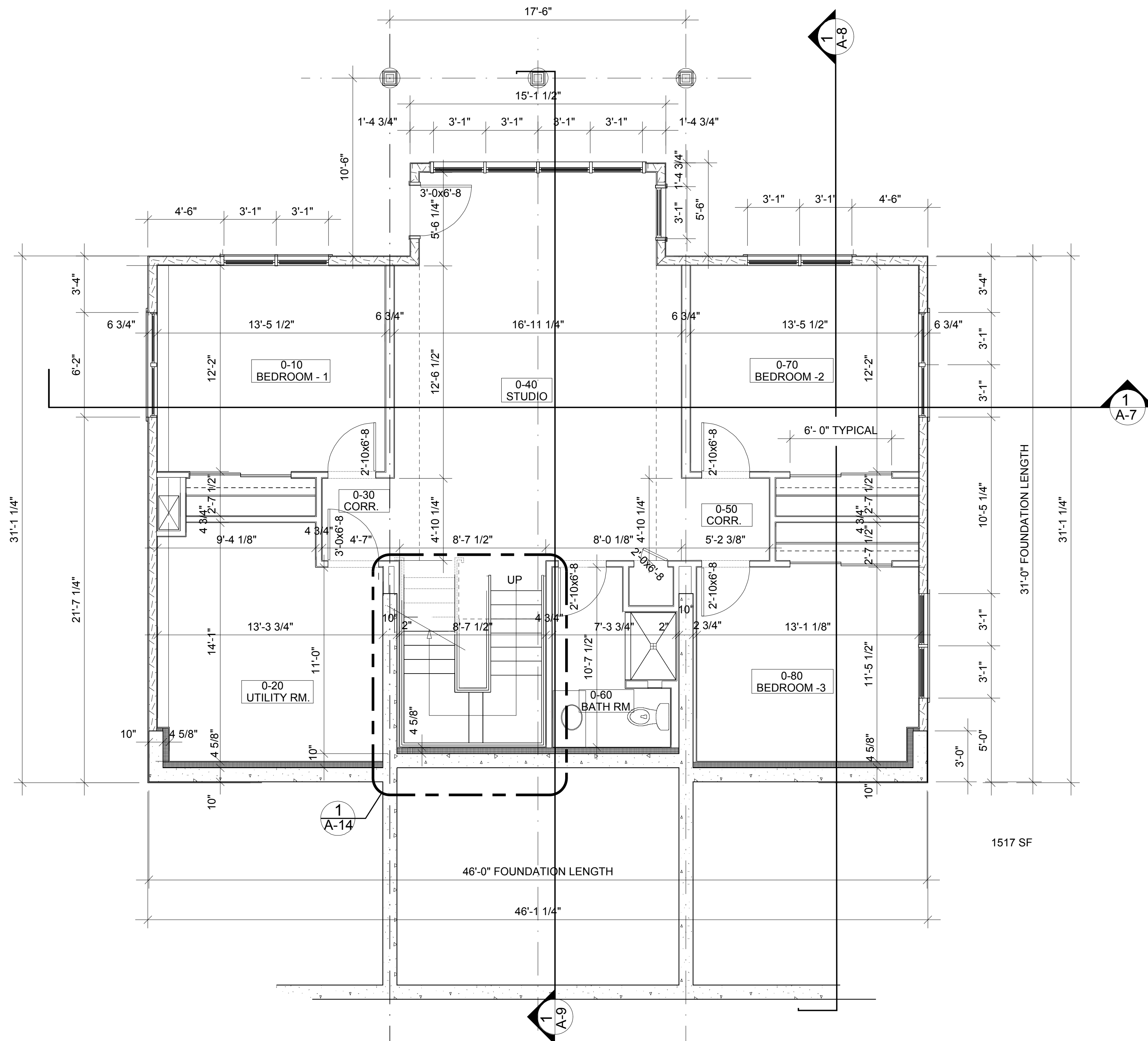
1 A-3 GROUND FLOOR PLAN Scale 1/4"=1'-0" LEV-LOWER_P1
