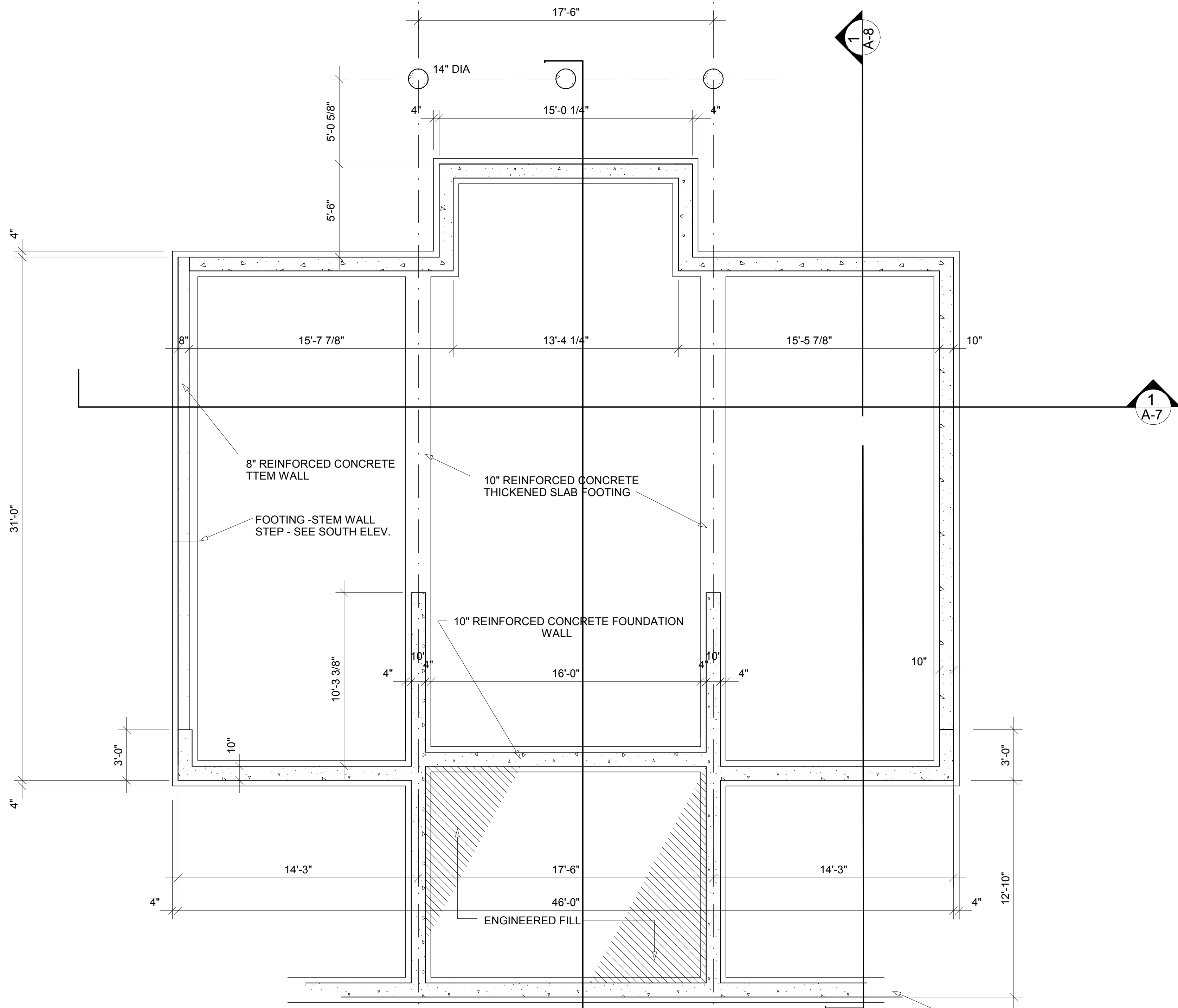
1 FOUNDATION PLAN A-2 Scale 1/4"=1'-0" LEV-LOWER_FDN-WALL
