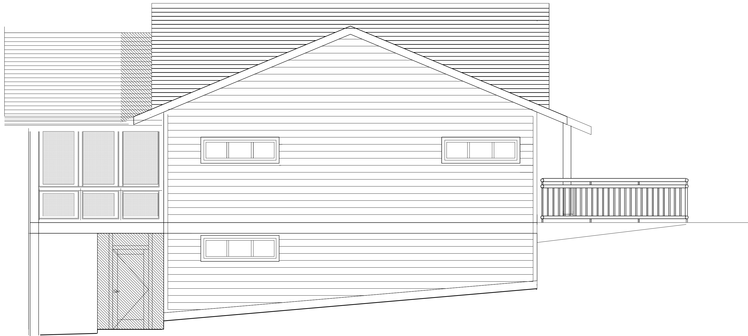
2 SOUTH ELEVATION A1.1 Scale 1/4"=1'-0" REV-SOUTH-01-25-18
