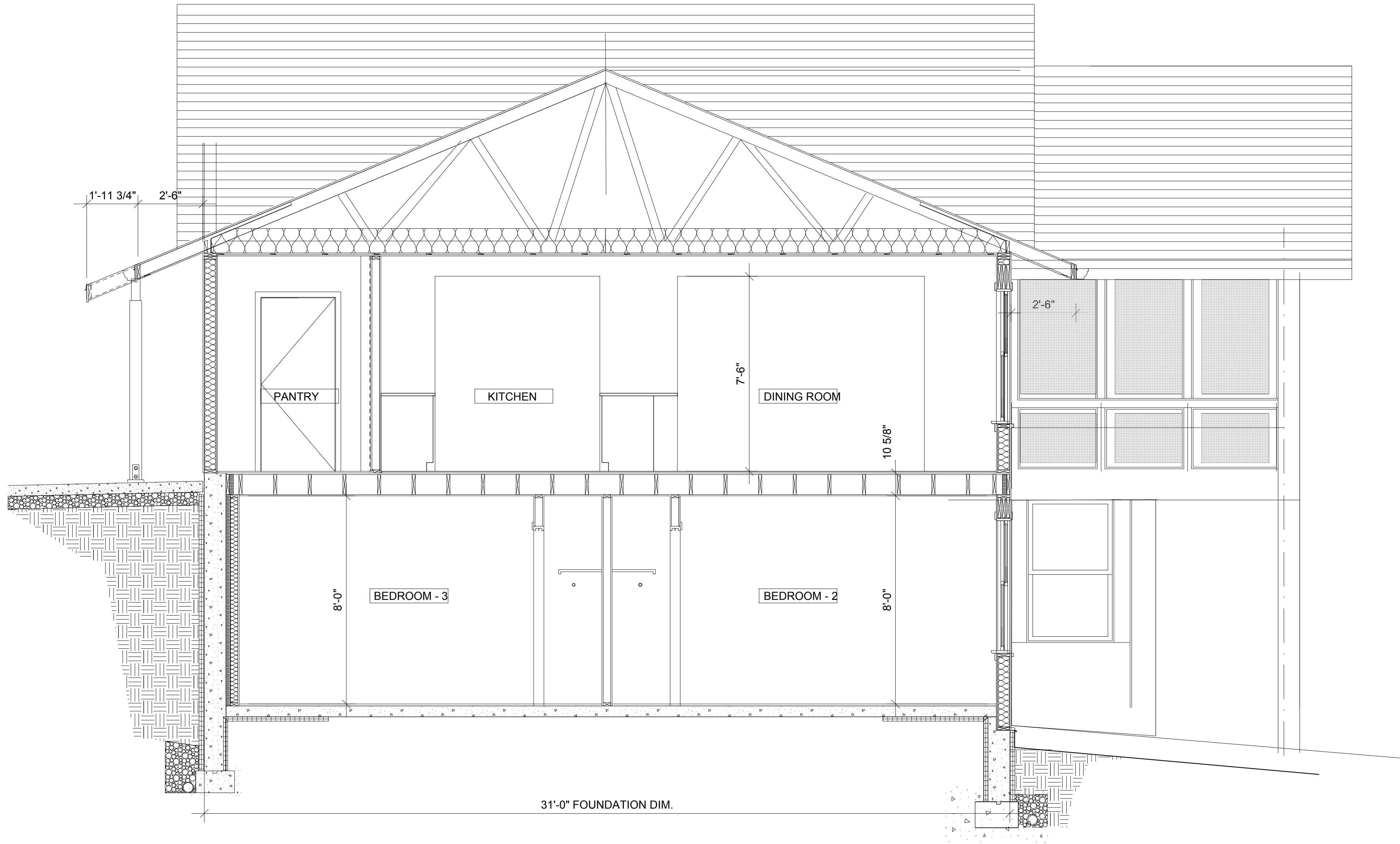
1 EAST - WEST -SECTION # 1 A1.1 Scale 3/8"=1'-0" E-W-SECT-1
