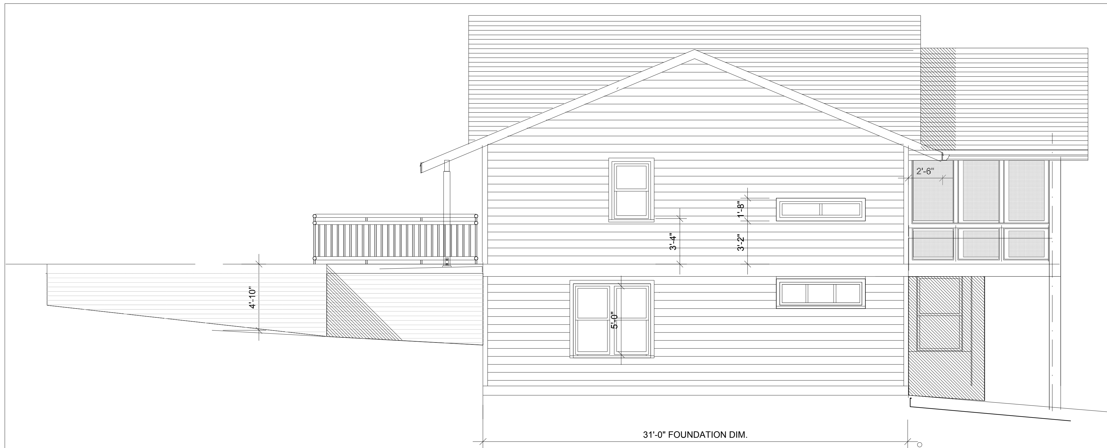
1 NORTH ELEVATION A1.1 Scale 1/4"=1'-0" NORTH --ELEV-BLDG-SECT
