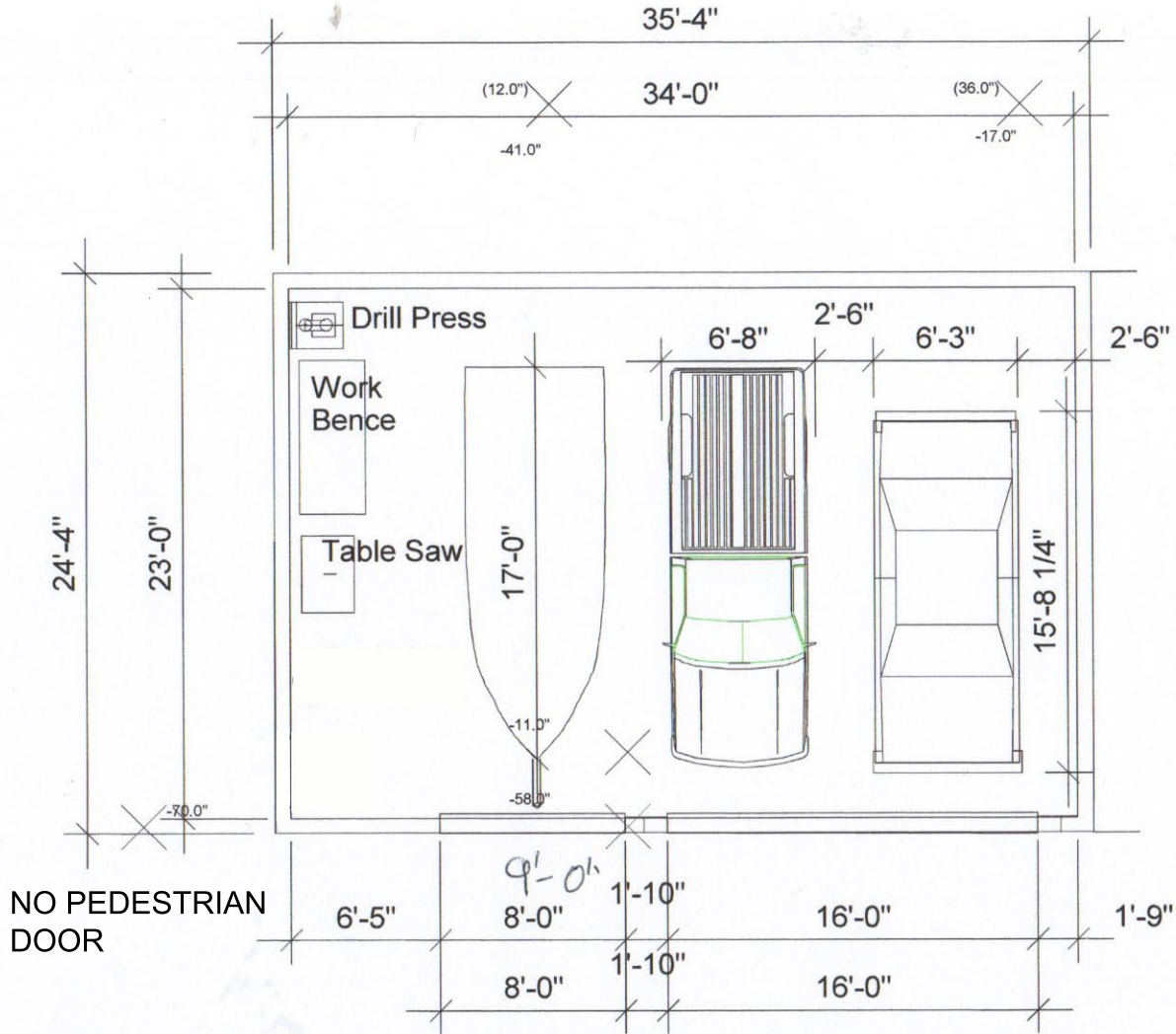
GARAGE PLAN 34' WIDE SCALE 1/8" = 1'-0"
